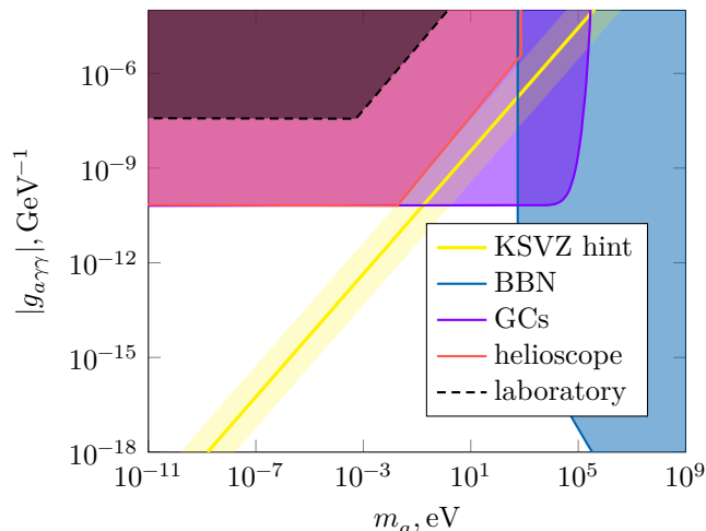
Figure 3.4: Summary of up-to-date (m_a, g_{a\gamma\gamma}) -space constraints for the axion. Shaded regions are excluded experimentally. The “hint” line indicates where KSVZ axions would be found. Many more experimental constraints exist; see [1, 5, 34] for more detailed exclusion plots.
