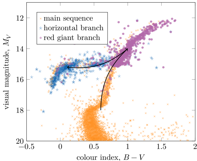
Figure 3.3: An example colour-magnitude plot for the Messier 5 globular cluster, showing main branches of stellar evolution. The visual magnitude encodes luminosity (increasing upwards) and the colour index encodes surface temperature (increasing right-to-left). Stellar evolution flows in the direction of the arrows. (Data from [37].)
